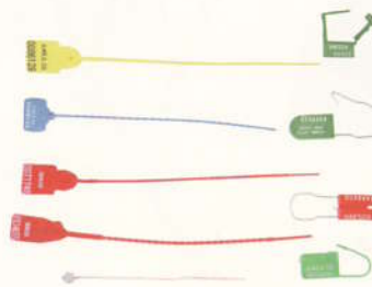
SEALS: PLASTIC PADLOCK
